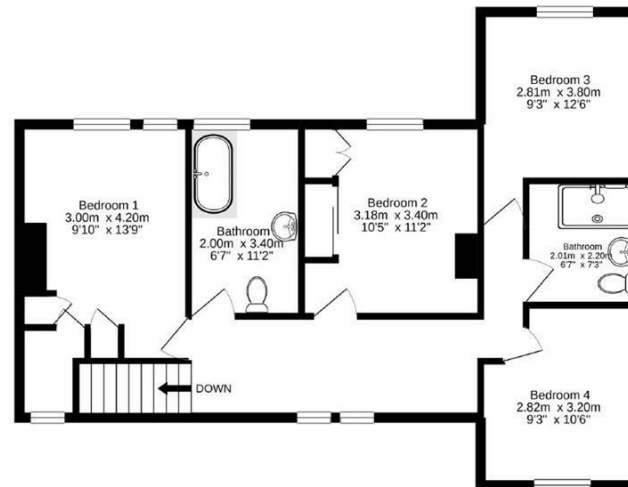
1st floor 65.4 sq.m. (704 sq.ft.) approx.
